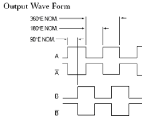
Figure 6: Output wave form of the encoders (taken from the specifications)
