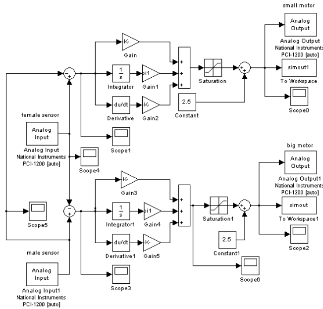
Figure 11: Control model
