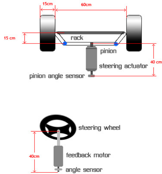
Figure 2: Components of a steer-by-wire system
