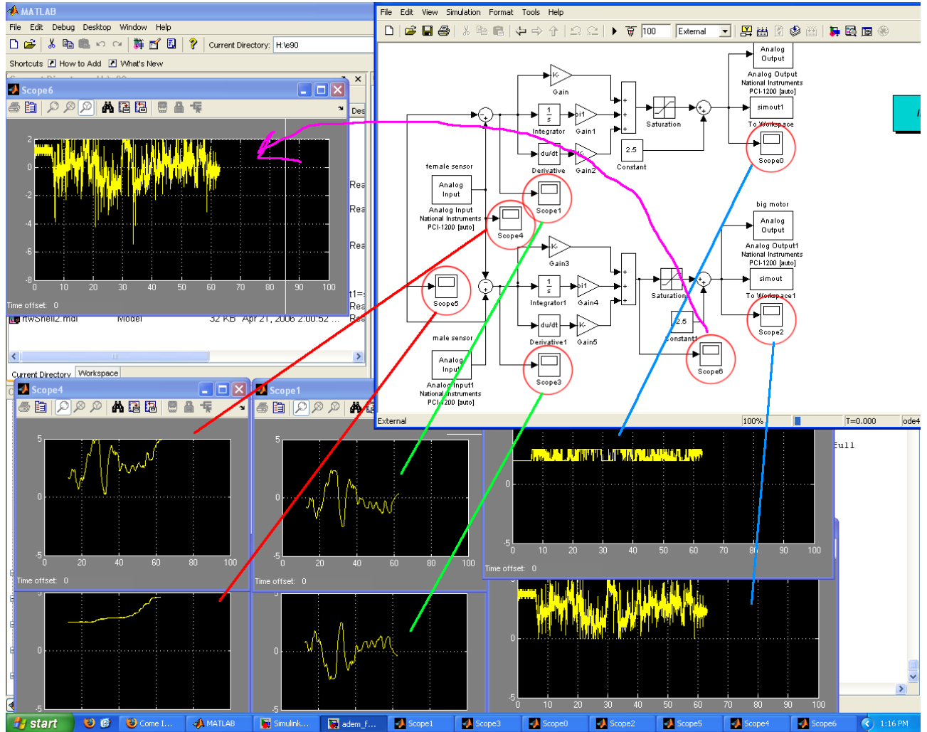
Figure 12: Sample operation Scope 0: Saturated feedback actuator output, Scope 1: error signal for feedback actuator, Scope 2: output for steering motor, Scope3: error signal for steering motor, Scope 4: input from feedback actuator sensor, Scope 5: input from steering angle sensor, Scope 6: Unsaturated output from steering motor PID
