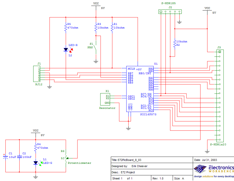
Figure 8: PIC microcontroller schematics (courtesy of Erik Cheever).
