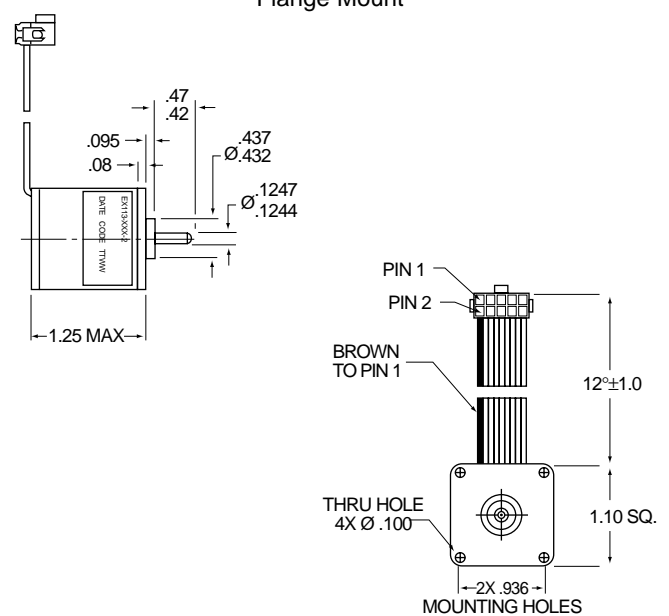
Flange Mount
