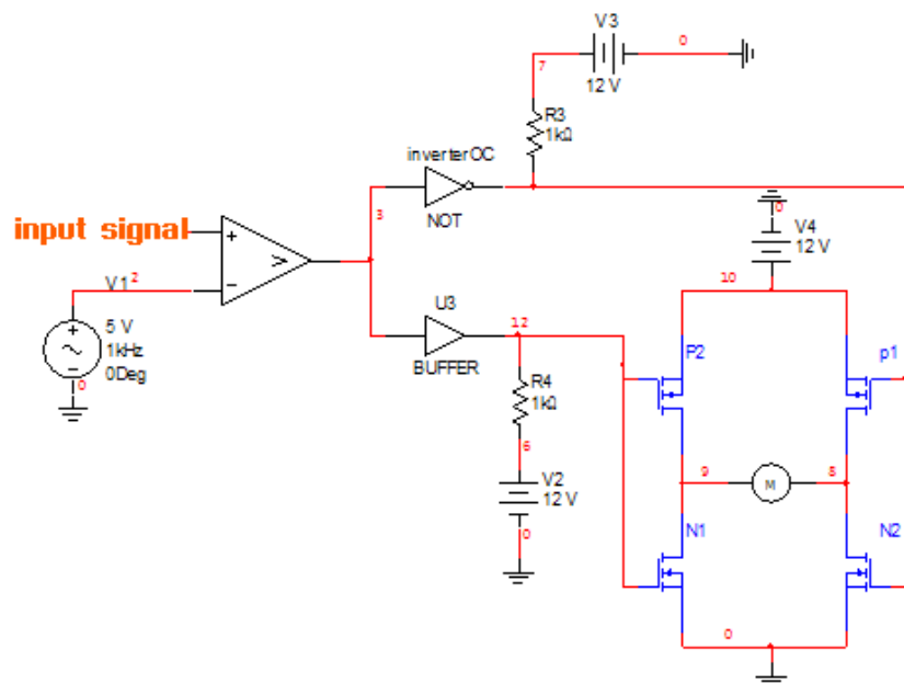
Figure 9: Pulse width modulation and the H-Bridge Configuration
