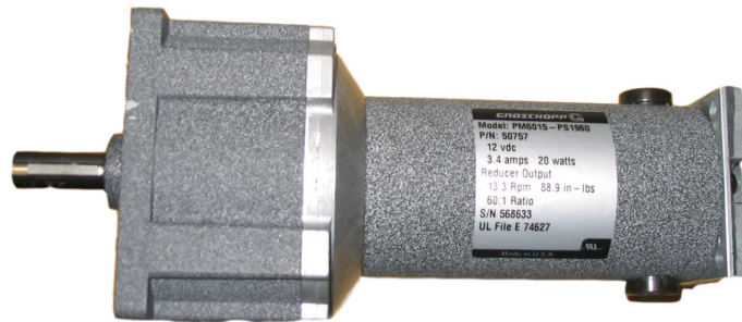
Figure 3: Steering Actuator
