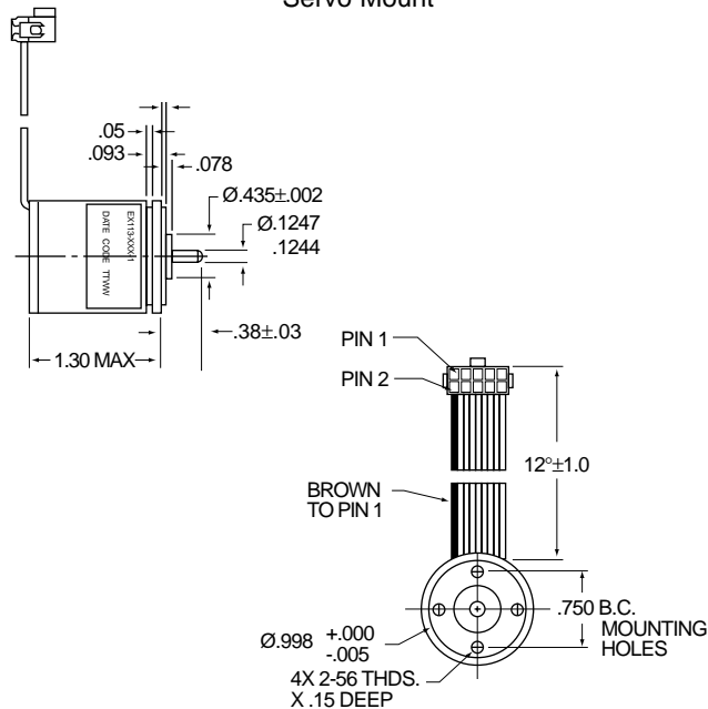
Servo Mount
